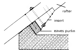
10 Detail at foot of roof allowing rafters to overhang
